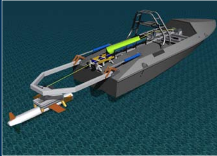
Towed Sonar LARS for USV
